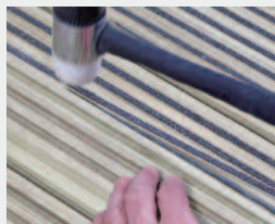
Fitting Q-Grip® strip (see pages 37)
